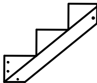
(2) SR1 - STAIR STRINGER ASSEMBLY - W2A02074 1"x8 5/8"x31 5/8" (24x220x802)
