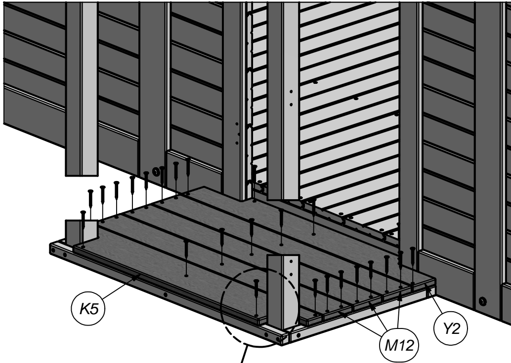
(3) M12 - PORCH BOARD - W4L07441 5/8"x3 3/8"x29 1/8" (16x86x740)
