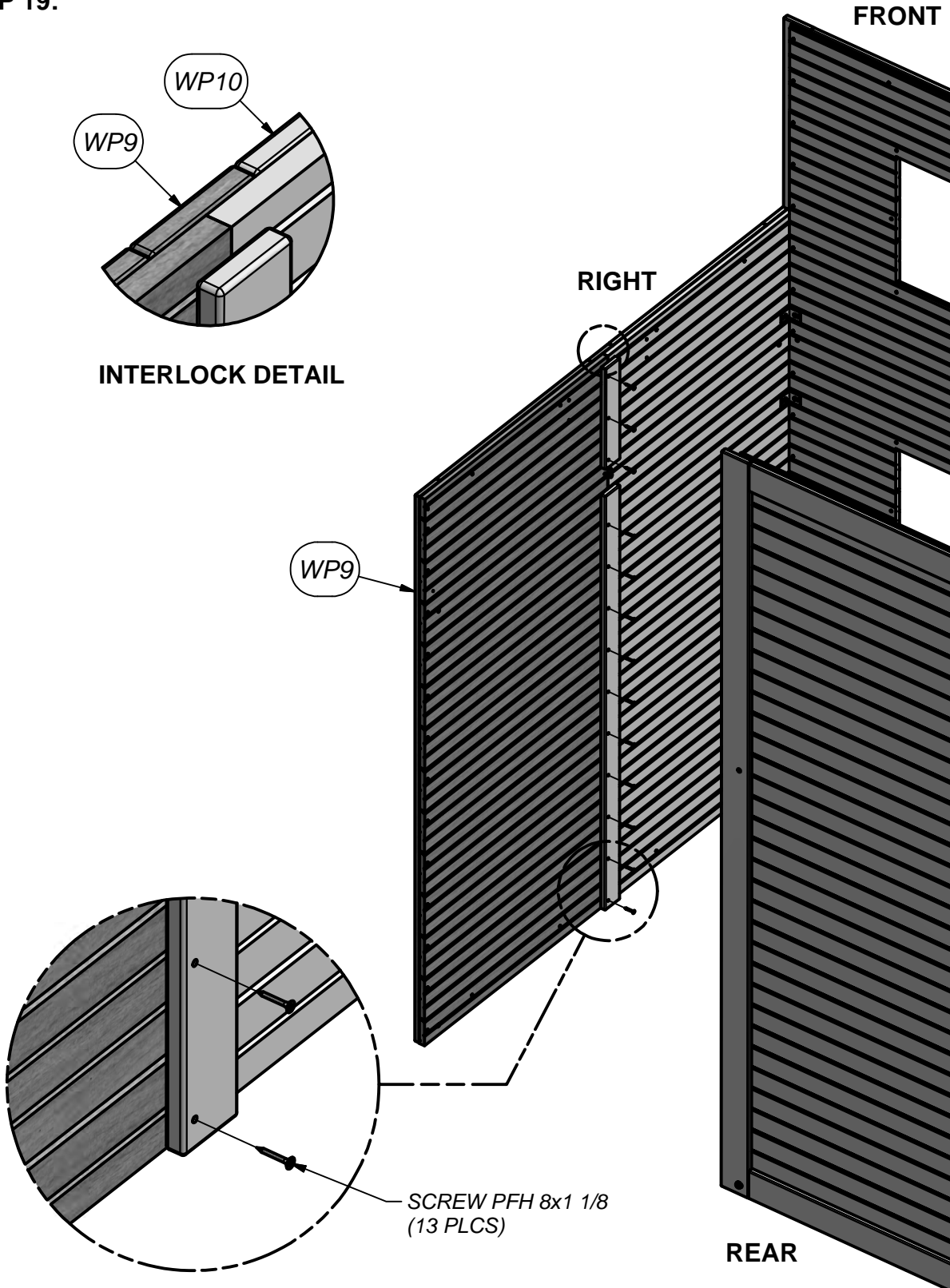
(1) WP9 - RIGHT SIDE REAR PANEL - W2A02058 1 7/8"x31 1/8"x66 1/2" (48x789x1690)
