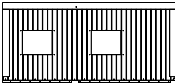
(1) WP1 - FRONT RIGHT WALL PANEL - W2A02050 1 7/8"x41 1/8"x89 1/2" (48x1043x2273)
