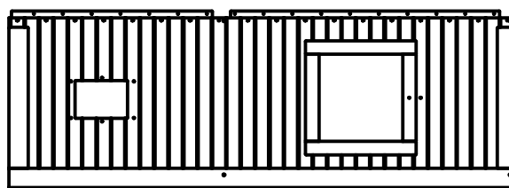
(1) WP6 - REAR LEFT WALL PANEL - W2A02055 1 7/8"x41 1/8"x89 1/2" (48x1044x2273)
