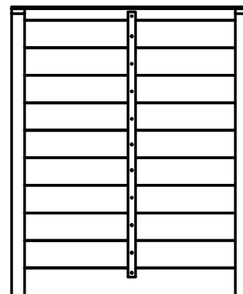
(2) RP2 - CENTER ROOF PANEL - W2A02064 1 5/8"x43 1/2"x53 3/8" (42x1102x1354)
