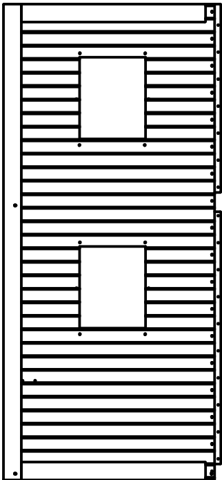
(1) WP3 - FRONT LEFT WALL PANEL - W2A02052 1 7/8"x41 1/8"x89 1/2" (48x1043x2273)
