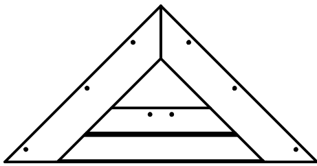
(1) GP2 - GABLE END ASSEMBLY - W2A02062 1 1/4"x28 3/8"x14 1/4" (32x721x361)
