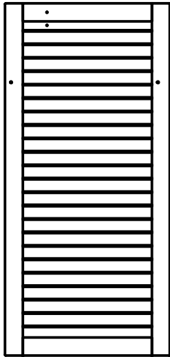
(1) WP9 - RIGHT SIDE REAR PANEL - W2A02058 1 1/4"x31 1/8"x66 1/2" (32x792x1690)
