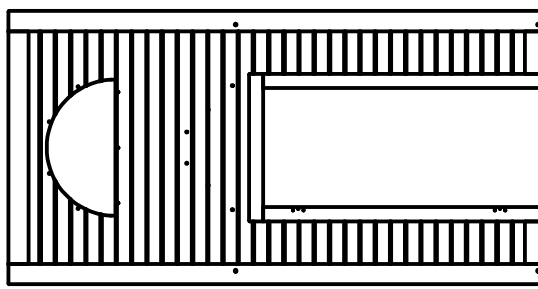
(1) WP2 - FRONT CENTER WALL PANEL - W2A02051 1 1/4"x45 1/2"x89 1/2" (32x1155x2273)
