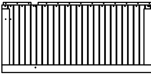
(1) WP10 - RIGHT SIDE FRONT PANEL - W2A02059 1 7/8"x31 1/8"x66 1/2" (48x789x1690)
