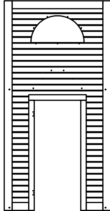
(1) WP2 - FRONT CENTER WALL PANEL - W2A02051 1 1/4"x45 1/2"x89 1/2" (32x1155x2273)
