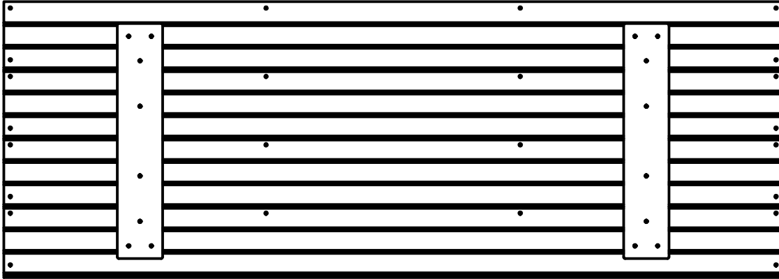
(3) FP1 - FLOOR PANEL - W2A02047 1 1/4"x20 1/2"x58 1/8" (32x516x1476)
