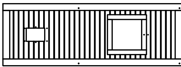
(1) WP4 - LEFT SIDE FRONT PANEL - W2A02053 1 1/4"x31 1/8"x89 1/2" (32x792x2273)
