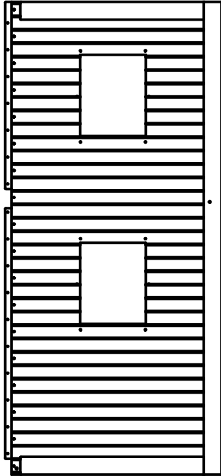
(1) WP1 - FRONT RIGHT WALL PANEL - W2A02050 1 7/8"x41 1/8"x89 1/2" (48x1043x2273)
