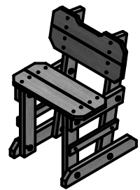
(1) WOODEN CHAIR - A4M00707
