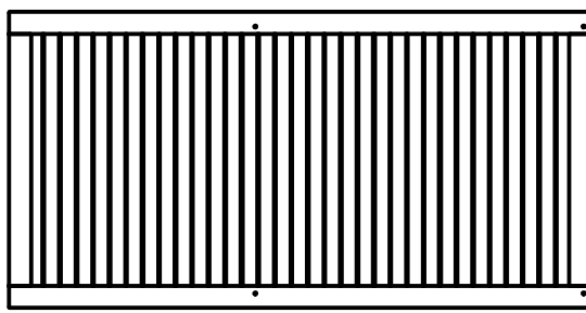
(1) WP7 - REAR CENTER WALL PANEL - W2A02056 1 1/4"x45 1/2"x89 1/2" (32x1155x2273)
