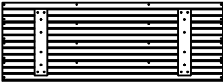
(1) FP1 - FLOOR PANEL - W2A02047 1 1/4"x20 1/2"x58 1/8" (32x516x1476)
