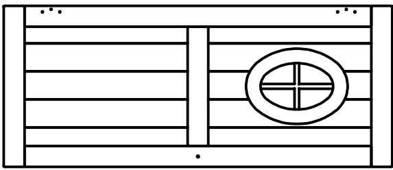
(1) DP1 - FRONT DOOR PANEL - W2A02060 1 1/8"x16 1/2"x43 7/8" (27x465x1124)
