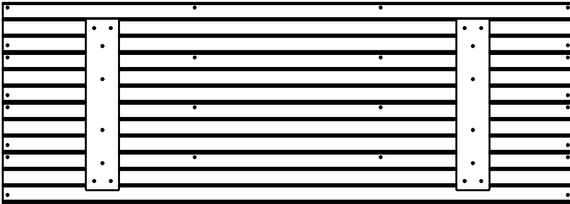
(2) FP2 - FLOOR PANEL - W2A02048 1 1/4"x20 1/2"x58 1/8" (32x523x1476)
