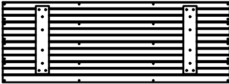
(2) FP4 - FLOOR PANEL - W2A02071 1 1/4"x20 1/2"x58 1/8" (32x523x1476)
