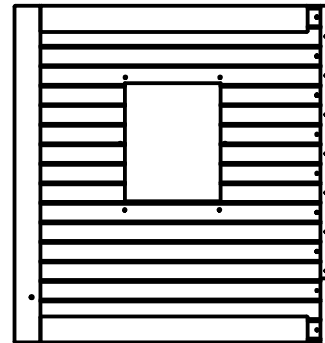
(1) WP8 - REAR RIGHT WALL PANEL - W2A02057 1 7/8"x41 1/8"x43 3/4" (48x1043x1112)
