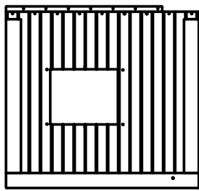
(1) WP8 - REAR RIGHT WALL PANEL - W2A02057 1 7/8"x41 1/8"x43 3/4" (48x1043x1112)
