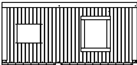
(1) WP5 - LEFT SIDE REAR PANEL - W2A02054 1 7/8"x31 1/8"x89 1/2" (48x789x2273)
