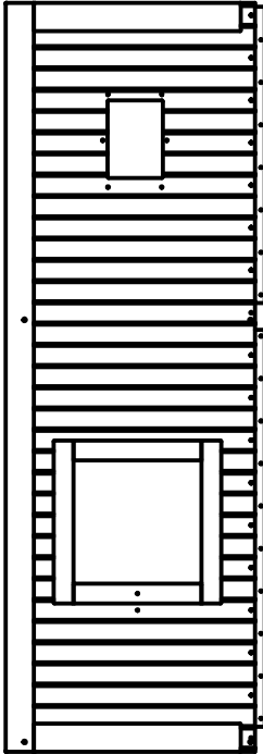
(1) WP5 - LEFT SIDE REAR PANEL - W2A02054 1 7/8"x31 1/8"x89 1/2" (48x789x2273)
