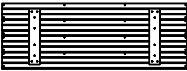
(1) FP1 - FLOOR PANEL - W2A02047 1 1/4"x20 1/2"x58 1/8" (32x516x1476)
