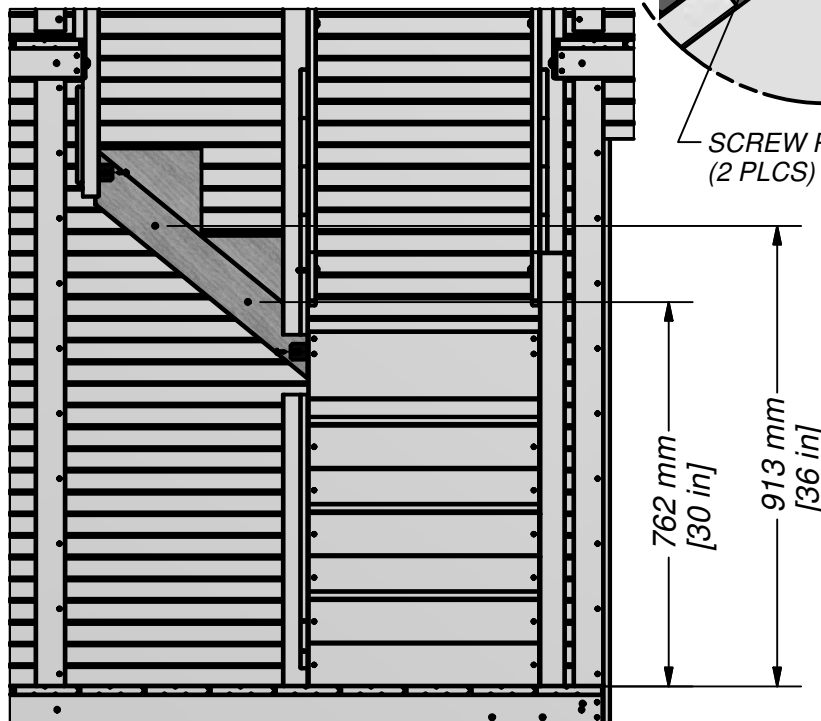
SCREW PFH 8x1 1/2 (2 PLCS)
