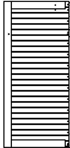
(1) WP10 - RIGHT SIDE FRONT PANEL - W2A02059 1 7/8"x31 1/8"x66 1/2" (48x789x1690)
