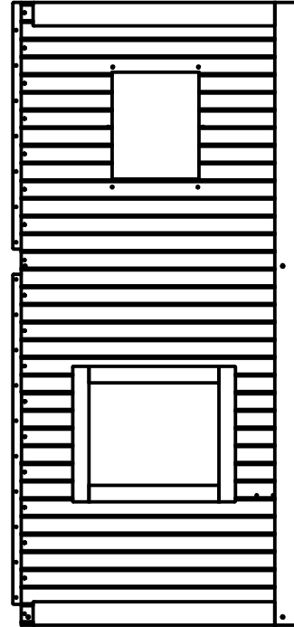
(1) WP6 - REAR LEFT WALL PANEL - W2A02055 1 7/8"x41 1/8"x89 1/2" (48x1044x2273)
