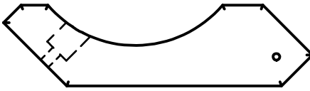
(2) J7 - PORCH CORBEL - W4L07230 1"x2 3/8"x9" (24x60x230)
