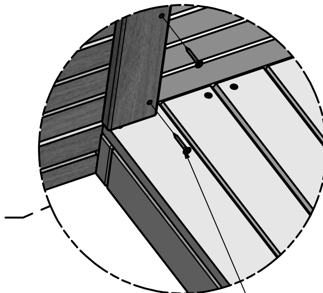
INTERLOCK DETAIL
