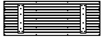
(1) FP3 - FLOOR PANEL - W2A02049 1 1/4"x20 1/2"x58 1/8" (32x523x1476)
