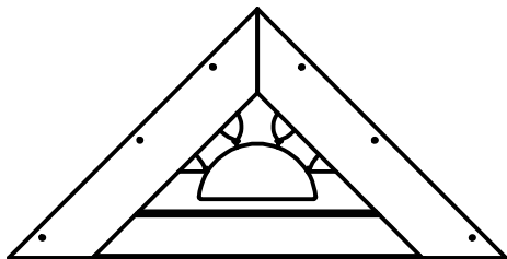
(1) PORCH GABLE END ASSEMBLY
