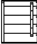
(1) RP3 - LEFT PORCH ROOF PANEL - W2A02068 1 5/8"x19 7/8"x23 7/8" (42x506x605)
