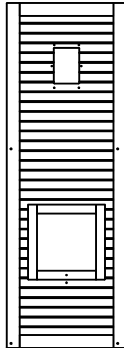
(1) WP4 - LEFT SIDE FRONT PANEL - W2A02053 1 1/4"x31 1/8"x89 1/2" (32x792x2273)
