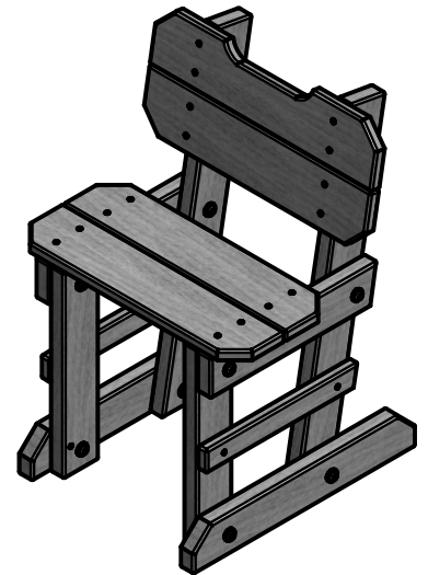
(1) WOODEN CHAIR - A4M00707
