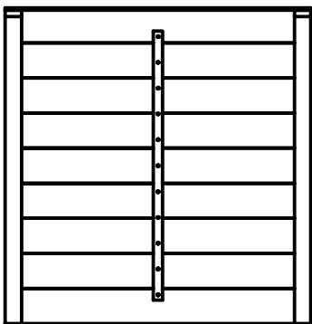
(4) RP1 - ROOF PANEL - W2A02063 1 5/8"x44"x45 7/8" (42x1118x1164)
