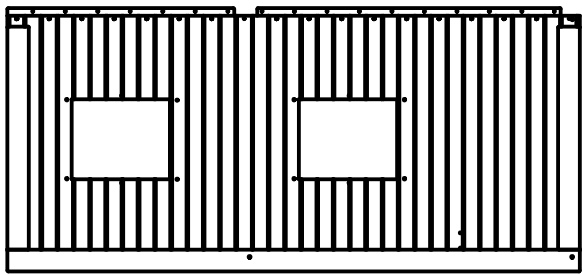
(1) WP3 - FRONT LEFT WALL PANEL - W2A02052 1 7/8"x41 1/8"x89 1/2" (48x1043x2273)
