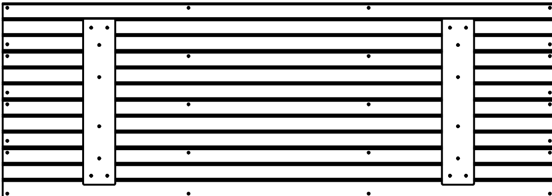
(1) FP3 - FLOOR PANEL - W2A02049 1 1/4"x20 1/2"x58 1/8" (32x523x1476)
