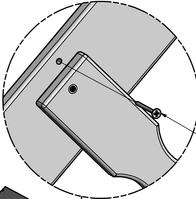
(2) RP1 - ROOF PANEL - W2A02063 1 5/8"x44"x45 7/8" (42x1118x1164)
