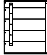
(1) RP4 - RIGHT PORCH ROOF PANEL - W2A02069 1 5/8"x19 7/8"x23 7/8" (42x506x605)
