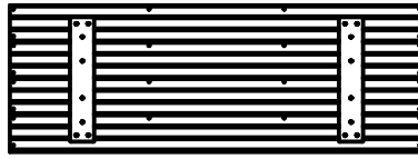
(2) FP2 - FLOOR PANEL - W2A02048 1 1/4"x20 1/2"x58 1/8" (32x523x1476)
