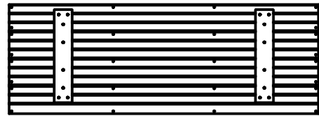
(1) FP4 - FLOOR PANEL - W2A02071 1 1/4"x20 1/2"x58 1/8" (32x523x1476)
